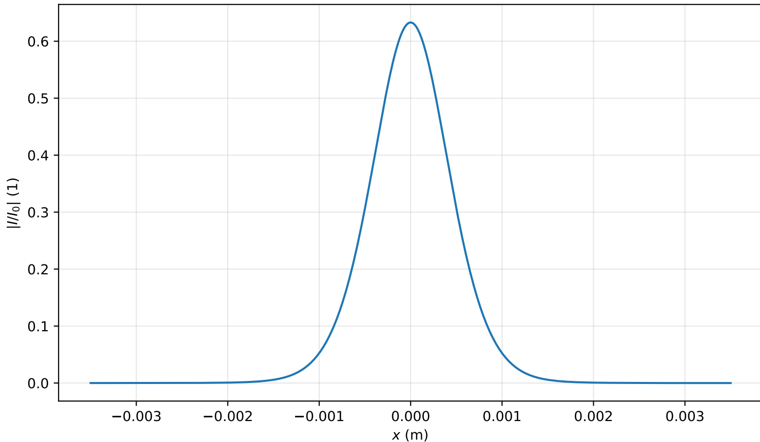
Intensity profile I(x, y = 0, z = 2.707m)/I_0 , P_{in}=0.5P_{cr} , artificial time
